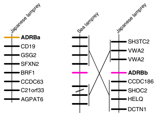
Fig. 3. Patterns of conserved synteny in the genomic regions that harbor \beta -adrenoreceptor genes in cyclostomes.
