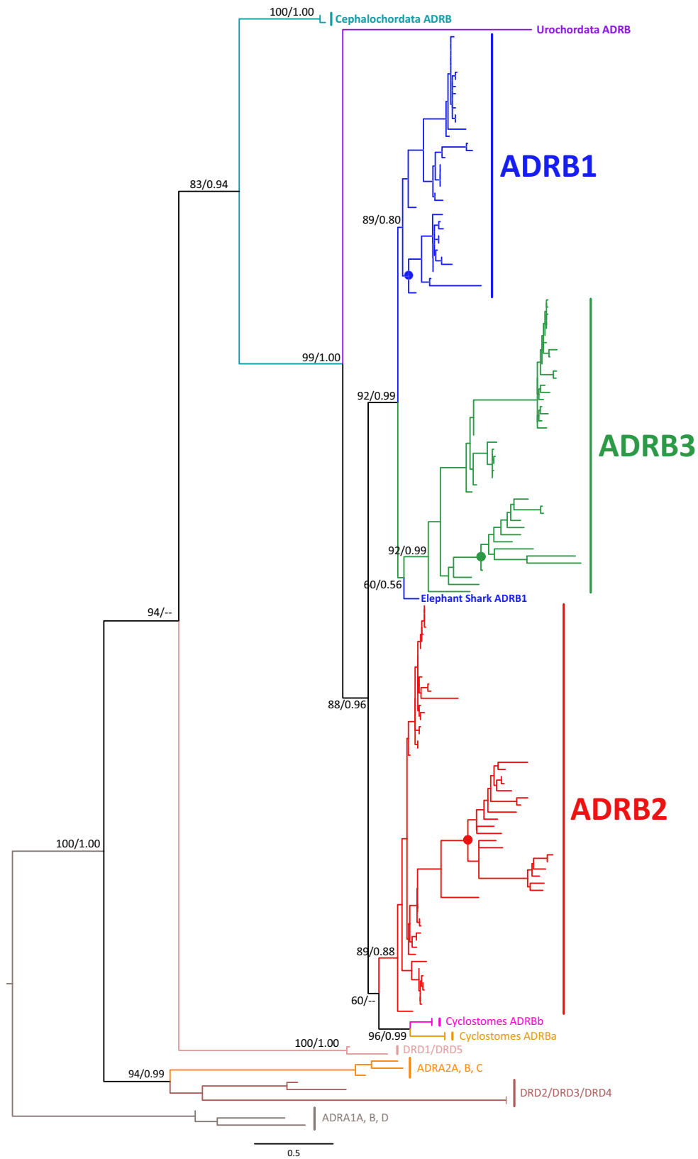
Fig. 1. Maximum likelihood phylogram depicting relationships among \beta -adrenoreceptors based on amino acid sequence data from transmembrane domains. Numbers on the nodes correspond to maximum likelihood ultrafast bootstrap and Bayesian posterior probabilities support values. Color dots denote the fish subtrees that are expanded in Fig. 4. (For interpretation of the references to colour in this figure legend, the reader is referred to the web version of this article.)
