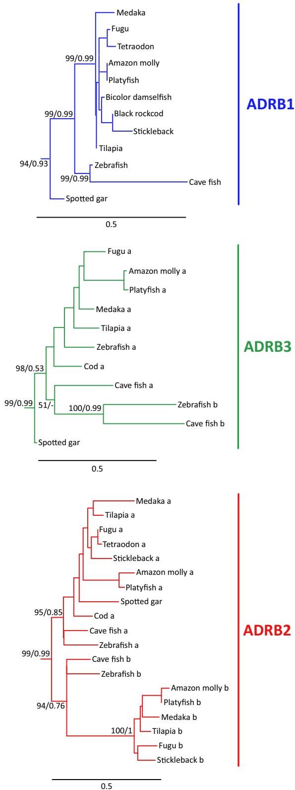
Fig. 4. Maximum likelihood phylogenetic relationships among \beta -adrenoreceptors in fish. Upper panel: phylogenetic relationships among ADRB1 sequences of fish. Middle panel: phylogenetic relationships among ADRB3 sequences of fish. Lower panel: phylogenetic relationships among ADRB2 sequences of fish. Numbers on the nodes correspond to maximum likelihood ultrafast bootstrap and Bayesian posterior probabilities support values. These topologies do not represent novel phylogenetic analyses; they are the fish clades that were recovered from Fig. 1.
