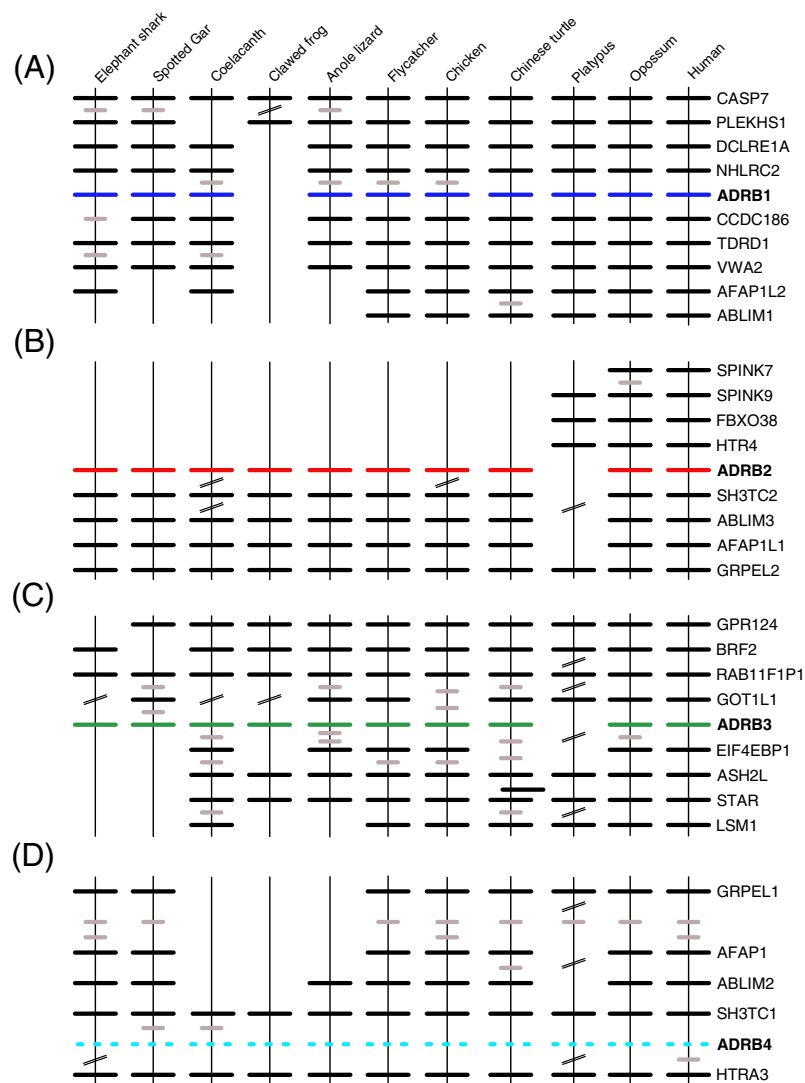
Fig. 2. Patterns of conserved synteny in the genomic regions that harbor \beta -adrenoreceptor genes in gnathostome vertebrates. A) genomic region that harbors ADRB1 genes. B) Genomic region that harbors the ADRB2 genes. C) Genomic region that harbors the ADRB3 genes. D) Patterns of conserved synteny in the genomic region that would be the putative location of the fourth \beta -adrenoreceptor gene in gnathostome vertebrates. Asterisks in the lower panel denote that the orientation of the genomic piece is from 3' to 5'.
